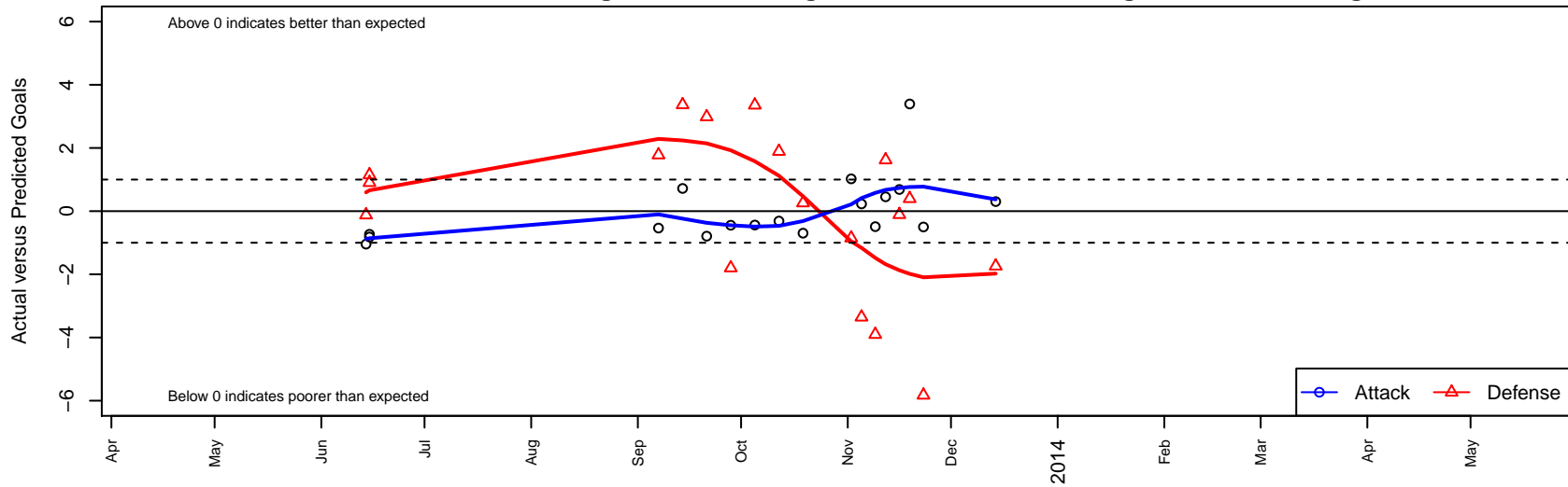
TBSC Arsenal FC B99 Dots are actual minus expected GF (blue circles) and GA (red triangles). Blue line is smoothed change in attack strength. Red is smoothed change in defense strength.
